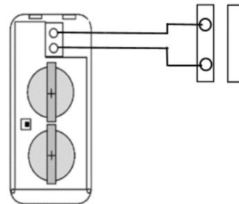
Figure 2: External contact
